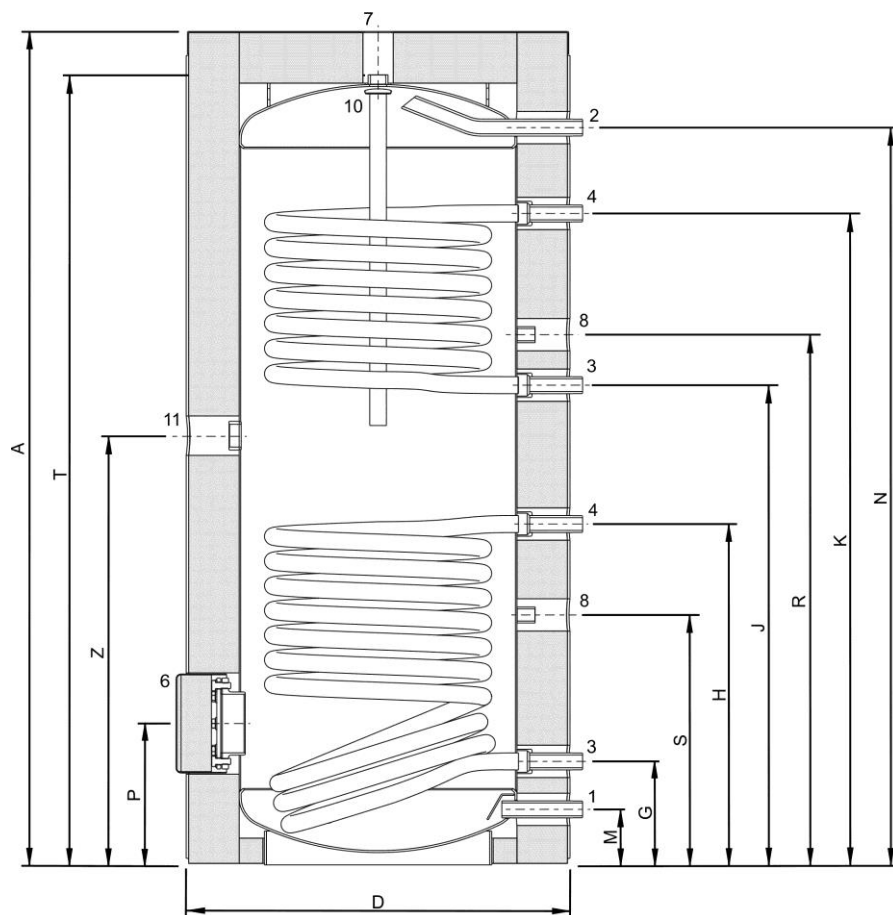
Front sectional view of the appliance
