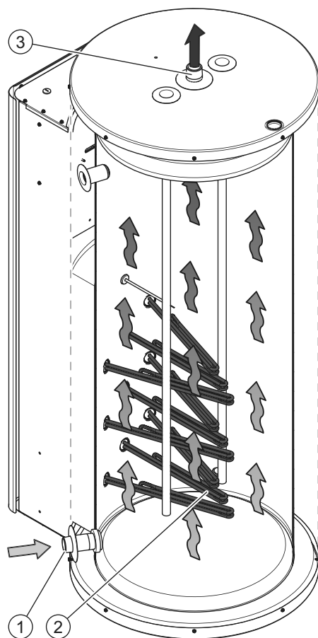
Illustration : chauffe-eau DRE
