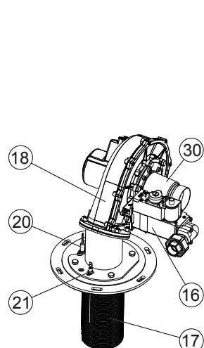
Illustration : Chauffe-eau SGS 80, 100, 120
