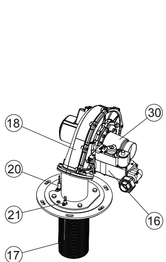
Fig. Boiler BFC 80, 100, 120
