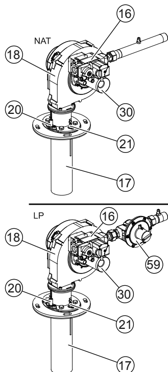
Fig. Boiler BFC 28, 30, 50, 60
