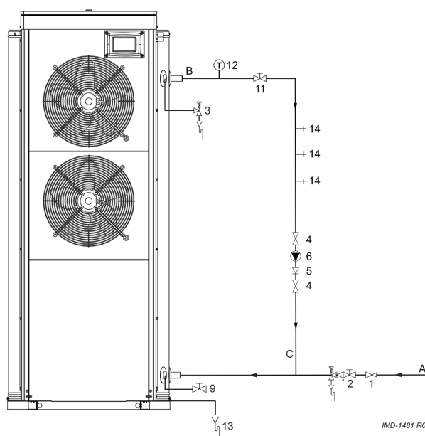
Fig. Installation diagram
