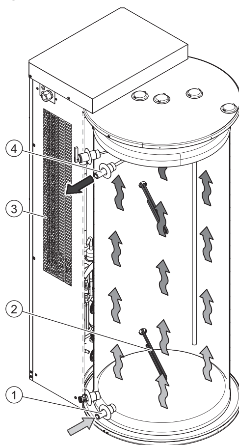
Fig. CAWH water heater
