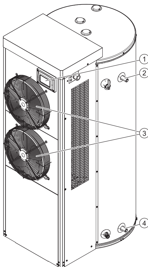
Afb. CAWH-boiler
