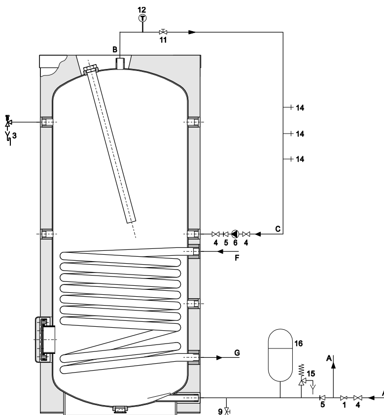
Installation Diagram
