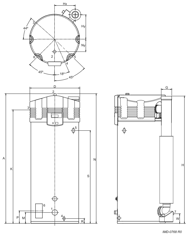
Fig. Dimensiones BFC 28, 30, 50, 60
