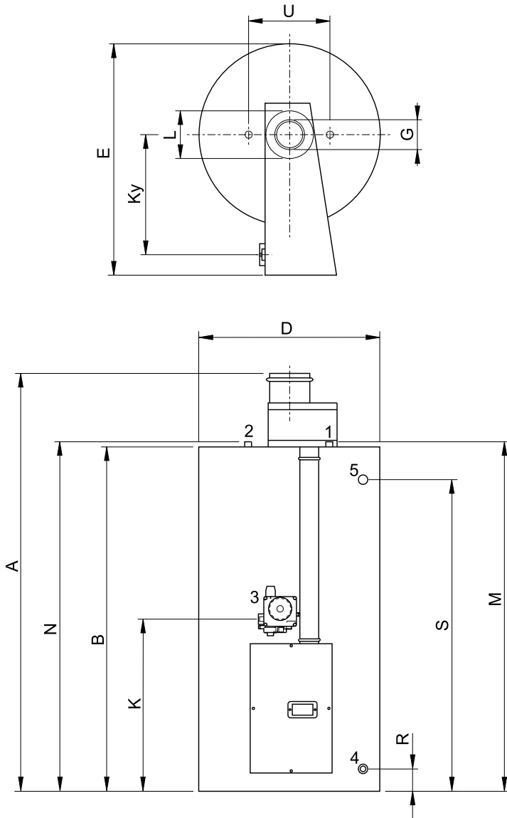
Figure 2 - Dimensions
