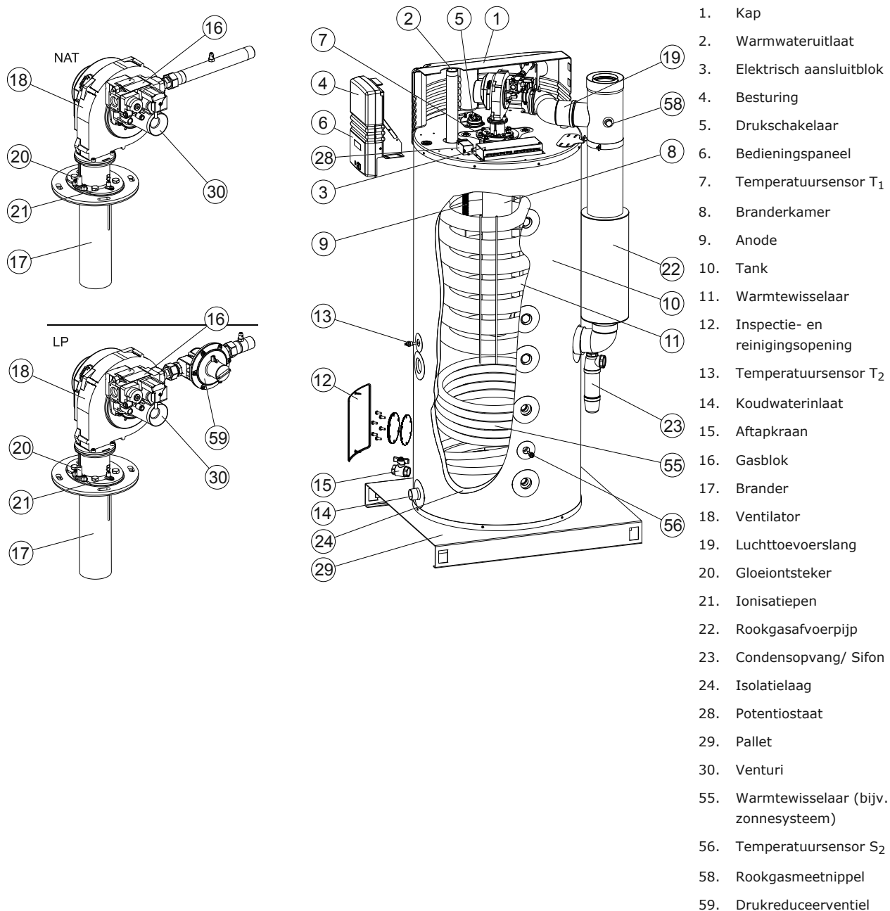
Afb. SGE-boiler
