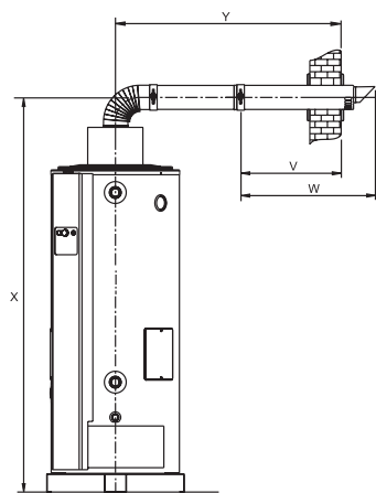
Evacuation coaxiale murale
